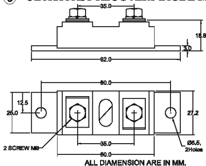
ULTRA FAST RECOVERY DIODE MODULE
