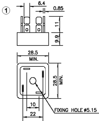
ULTRA FAST RECOVERY DIODE MODULE
